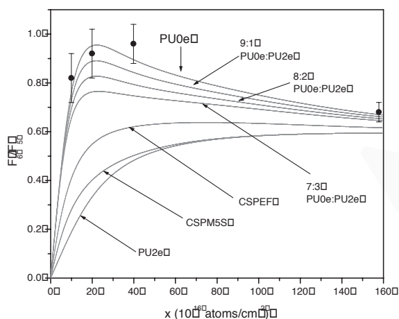
Fig. 1. Ratio of 6^+ : 5^+ charge states in the recoils of ^{12}\text{C}(\alpha, \gamma)^{16}\text{O} as a function of target thickness. The solid lines are different models of electron pick-up or loss during the nuclear capture. PU0E has 0 electrons of the He atom picked up by the O recoil, PU2E has 2 electrons picked up.
