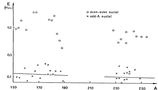
Figure 6: Excitation energy-gap in even-even nuclei compared to odd-mass nuclei[2].
