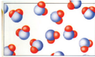
Figure 1: Steam is fully symmetric.
