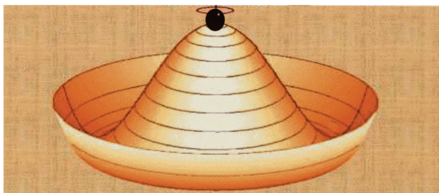
Figure 3: Mexican hat potential. The ball rolls down into the brim breaking the initial “symmetric state”.
