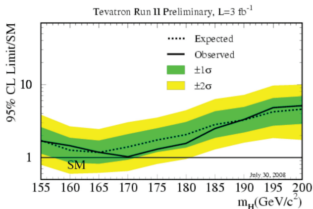
Figure 4: Exclusion plot for SM Higgs boson.
