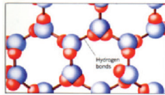
Figure 2: The snowflake has less symmetry than steam.
