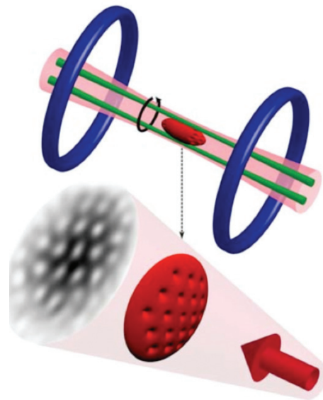
Figure 5: Superfluid vortices in trapped ultra cold atoms[1].
