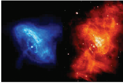
Figure 7: Crab pulsar in X-ray and optical: Superfluidity/superconductivity impacts cooling of neutron stars.
